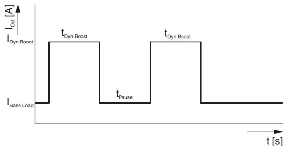
Figure 17 Basic curve of the dynamic boost process
